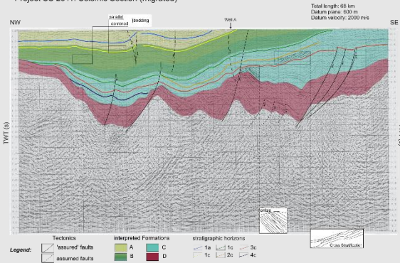
Project SS 2011: Seismic Section (migrated)
